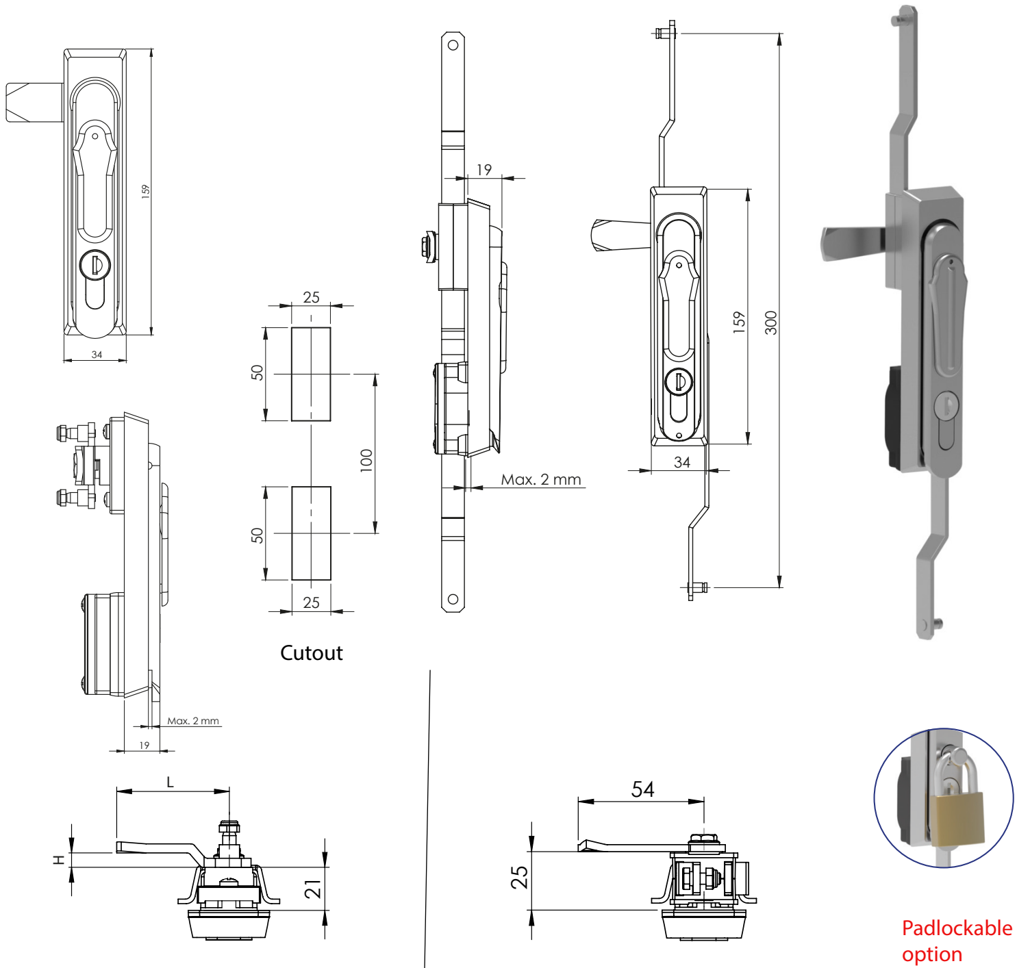
Version for 3 point cam - KK
