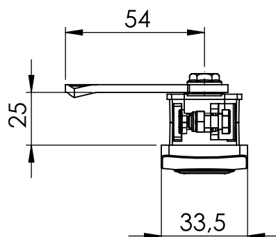
Version for cogwheel mechanism - M3
