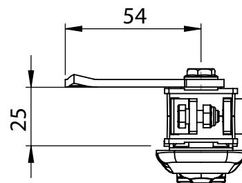
Version for cogwheel mechanism - M1
