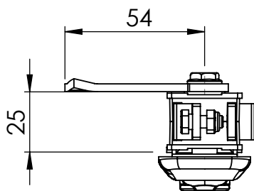
Version for cogwheel mechanism - M2
