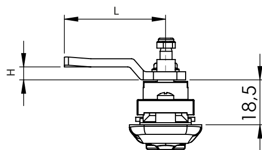
Version for 3 point cam - KK
